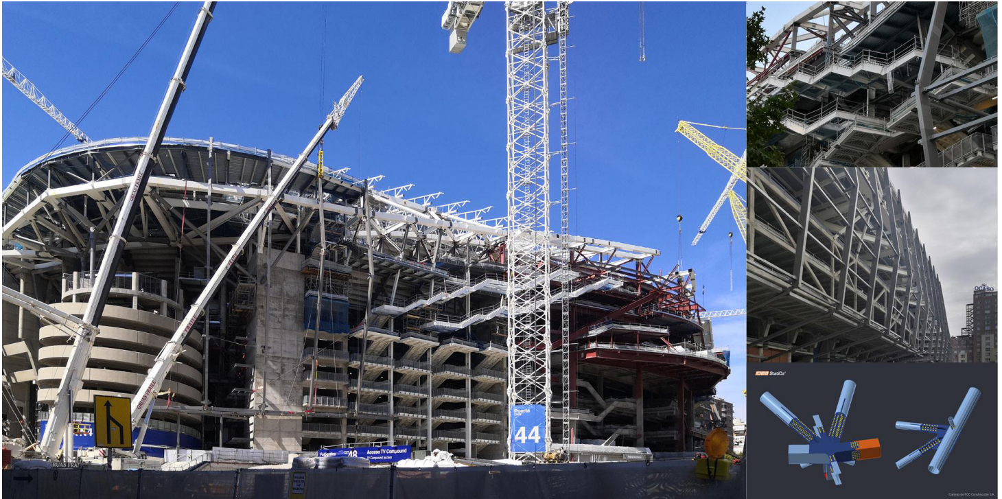
East Building, Façade and video scoreboard support structure
