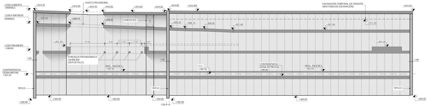
recalculation and analysis of deformations at Conde de Casal Station and recalculation of screens and slabs at Comillas Station
