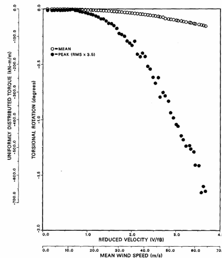
Elche Bridge - Torsional Response - Smooth Flow - \zeta = 0.055 Log. Dec.
